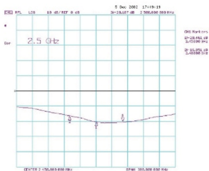
Return Loss
